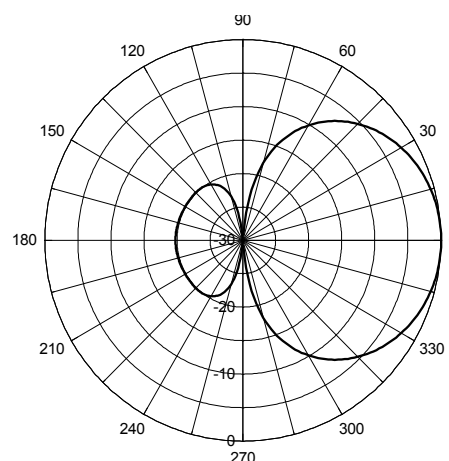
Diagrama de Radiação @160 MHz Plano – H Radiation Pattern @160 MHz – H Plane
