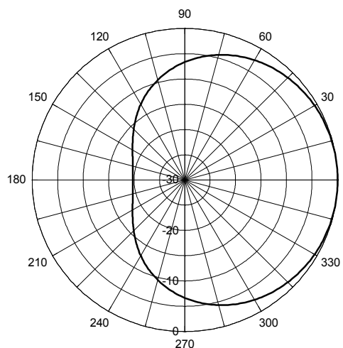
Diagrama de Radiação @160 MHz Plano – H Radiation Pattern @160 MHz – H Plane
