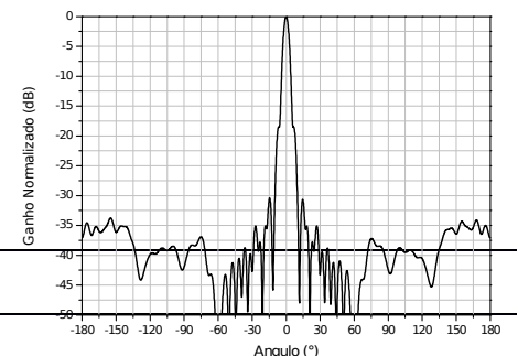
Diagrama de irradiação @ 2150 MHz Plano Vertical Vertical Plane Radiation Pattern @ 2150 MHz
